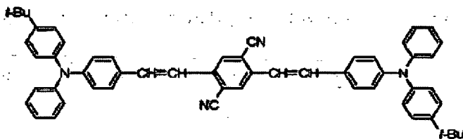
Structural formula (15)-6:
